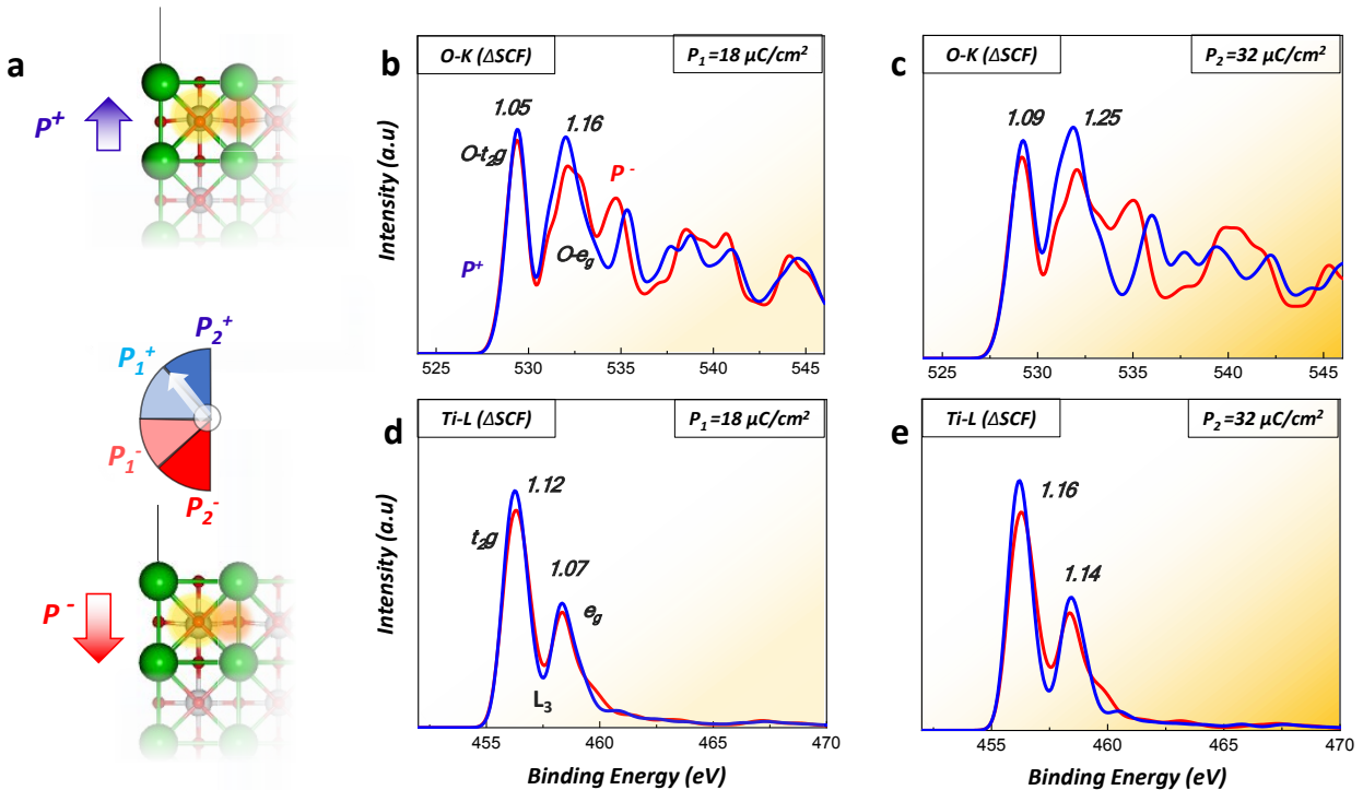
Figure 3. Excitations based on many-body, determinant \Delta SCF approach. (a) schematic of BaTiO 3 polarized slabs with upward and downward polarizations (b-c) O-K edge with t_{2g} and e_g peaks labeled with P_1 and P_2 polarization extent (d-e) Ti-L edge with t_{2g} and e_g peaks labeled with P_1 and P_2 polarization extent. Relative peak intensities between upward and downward polarized models ( P^+/P^- ) is noted on each peak.
