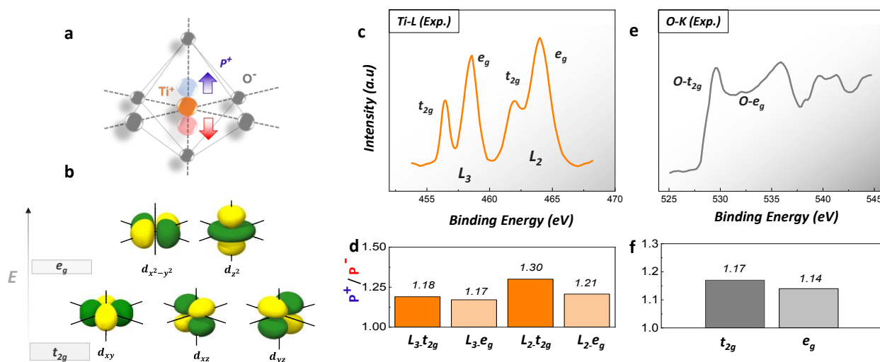
Figure 1. (a) Schematic TiO_6 octahedron within the BaTiO_3 tetragonal structure, with a Ti^+ cation in upward (blue) and downward (red) polarization states (b) possible hybridized orbitals between Ti-d and O-p states with d_z^2 and d_{x^2-y^2} on e_g and d_{xy} , d_{xz} or d_{yz} orbitals on t_{2g} states. Experimental XAS spectra and corresponding intensity ratios on each peak in upward vs downward positions on (c-d) Ti-L and (e-f) O-K edges of epitaxial BaTiO_3 .
