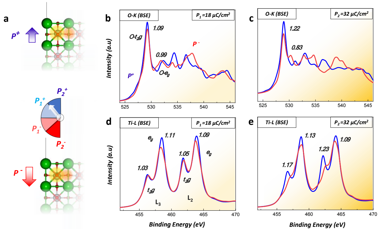
Figure 4. Excitations based on BSE approach. (a) schematic of BaTiO 3 polarized slabs with upward and downward polarizations (b-c) O-K edge with t 2g and e g peaks labeled with P 1 and P 2 polarization extent (d-e) Ti-L edge with t 2g and e g peaks labeled with P 1 and P 2 polarization extent. Relative peak intensities between upward and downward polarized models (P + /P - ) is noted on each peak in italic.
