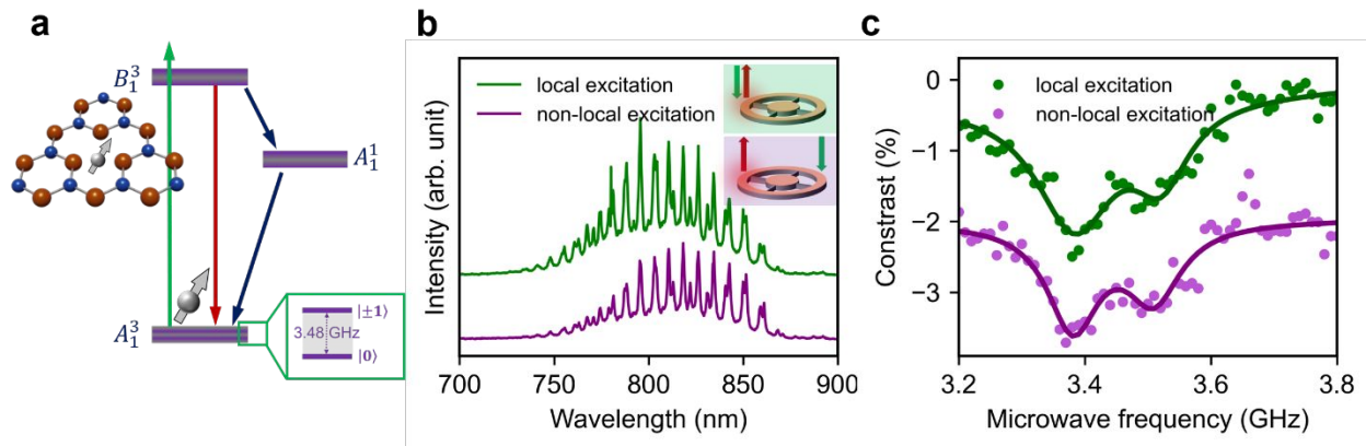
Figure 3. ODMR measurement of coupled V_B^- . (a) Schematic of the V_B^- defect and an energy diagram showing the main optical pumping cycle and the alternate cycle through the metastable state. (b) PL spectrum from coupled V_B^- in local and non-local configurations. The spectra were offset in Y-axis for clarity. The inset schematically shows these configurations. (c) ODMR measurement from coupled V_B^- in local and non-local configurations. The microwave power was set to 10 dB for both configurations. The ODMR contrast of the non-local excitation scheme was offset for clarity.
