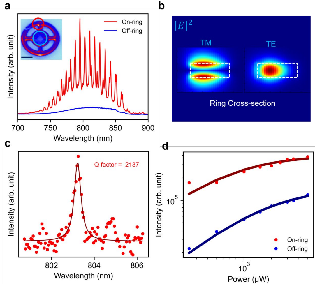
Figure 2. Optical characterization of the microring resonator. (a) PL spectrum collected on (red) and off (blue) the ring. Inset – confocal scanning image of the corresponding hybrid
