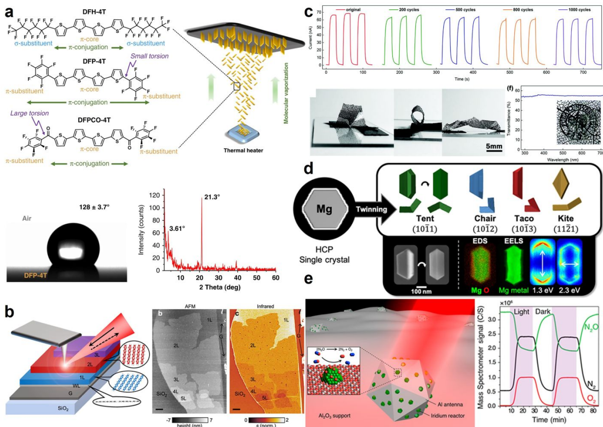
Figure 3: Recent demonstrations of function-enhanced plasmonic materials. a.) Schematic representation of the fabrication and characterization of fully organic nanostructured SERS films. Adapted from ref. 93 under creative commons attribution 4.0 http://creativecommons.org/licenses/by/4.0/ b.) Illustration and AFM topography of 2D graphene/pentacene heterostructured nanomaterials. Adapted from ref. 106 with permission from the American Chemical Society. c.) Chronoamperometry measurements under 350 nm illumination of bending cycles coupled with optical images of MXene UV photodetectors. Adapted from ref. 109 with permission from the Royal Society of Chemistry. d.) Cartoon representations, SEM images, and elemental analysis of twinned Mg nanoparticles. Adapted from ref. 73 e.) Schematic representation of AlIr nanoparticles and reactivity under irradiation measured via mass spectrometry. Adapted from ref. 47 with permission from the American Chemical Society.
