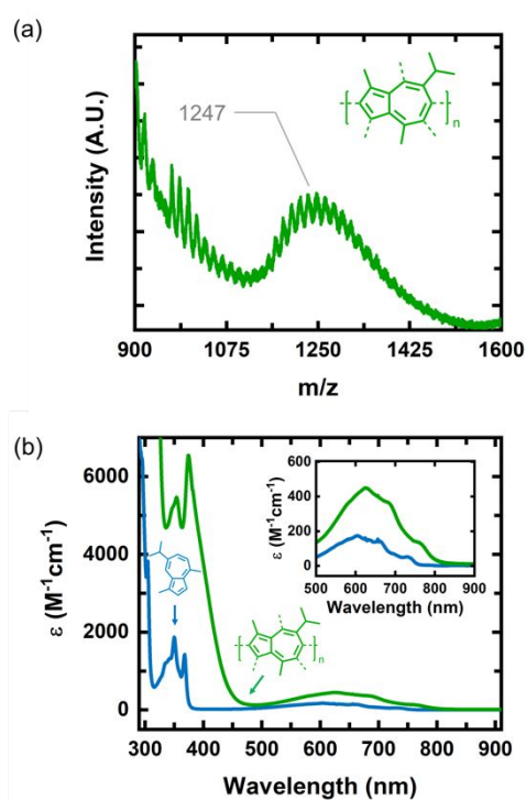
Figure 1. (a) LDI-MS of P1 oligomers synthesized via oxidative polymerization in CHCl 3 . (b) UV-vis spectra of monomer 1 (blue curve) and P1 oligomers (green curve) in hexane.
