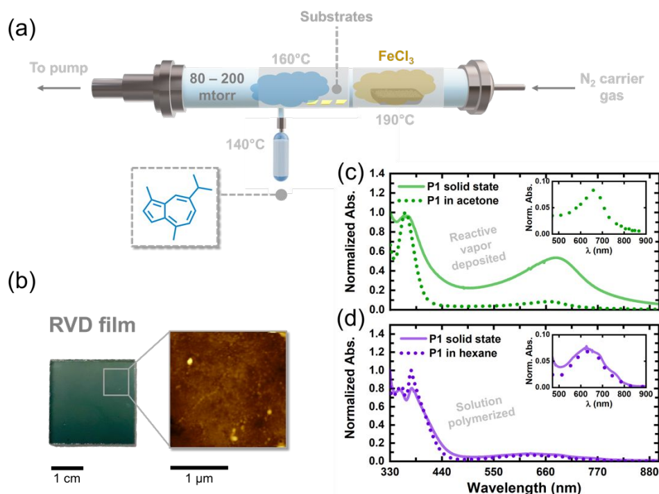
Figure 3. (a) Schematic of RVD reactor and conditions used for the vapor-phase polymerization of P1 . (b) Optical image of a rinsed RVD film (left) and corresponding AFM image (right) showing the topography of the film. (c) UV-vis spectra of RVD polymerized P1 measured in solution (dotted green line) and in the solid state (solid green line). (d) UV-vis spectra of solution polymerized P1 measured in solution (dotted purple line) and in the solid state (solid purple line).
