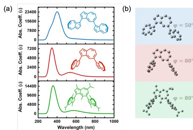
Figure 2. (a) Simulated UV-vis absorption spectra (TD-DFT, CAM-B3LYP/6-311G+) of guaiazulene and azulene trimers with varying torsion angles between repeat units. (b) 3D ball and stick models of the calculated structures with hydrogen atoms omitted for visual clarity.
