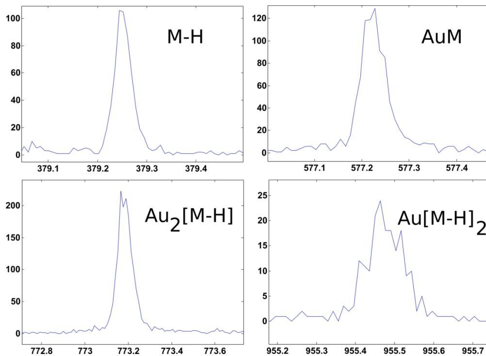
ToF-SIMS negative ion spectra from the PEG4thiol that show the characteristic molecular ion peaks from the PEG4thiol
