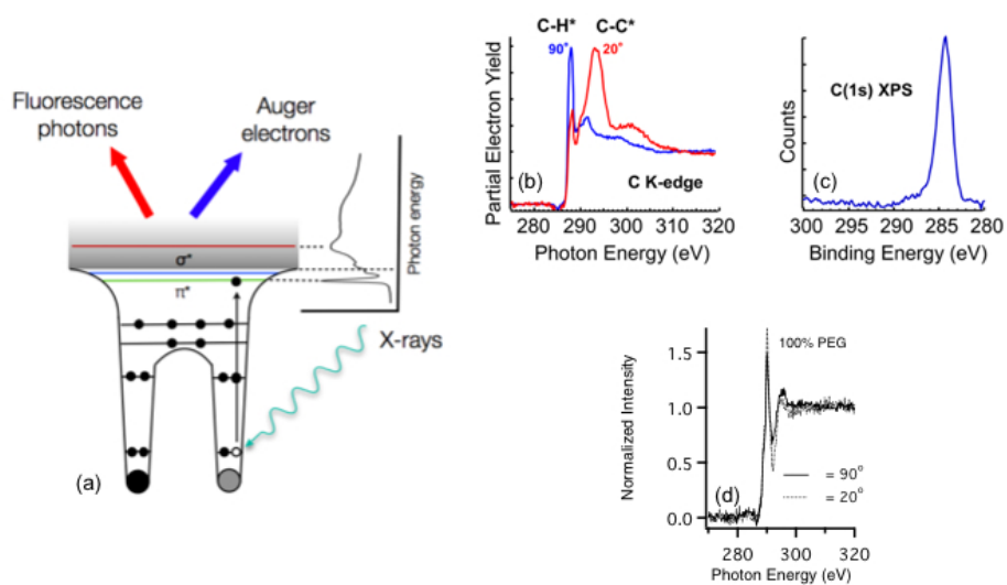
(a) Schematic of the photoexcitation process that takes place during a NEXAFS experiment. NEXAFS carbon K-edge (b) and XPS C1s (c) spectra acquired from an MHD SAM on gold. NEXAFS carbon K-edge spectra (d) of the PEG4thiol SAM acquired at x-ray incident angles of 90 and 20 degrees from the surface plane.
