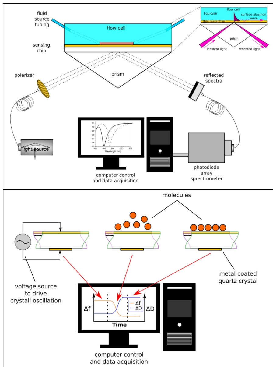
Schematic diagrams of wavelength SPR (top) and QCM-D (bottom) biosensing processes.
