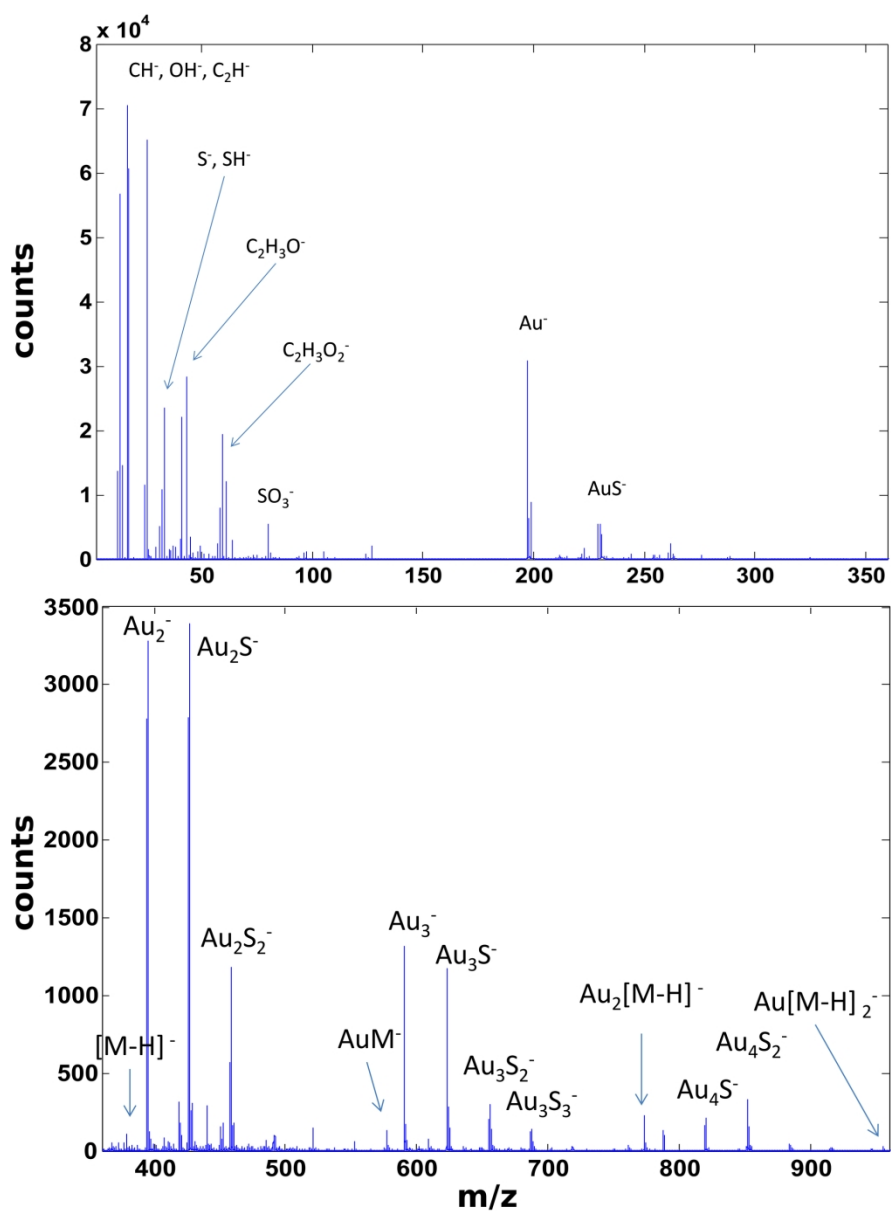
ToF-SIMS negative ion spectrum from the PEG4thiol SAM.
