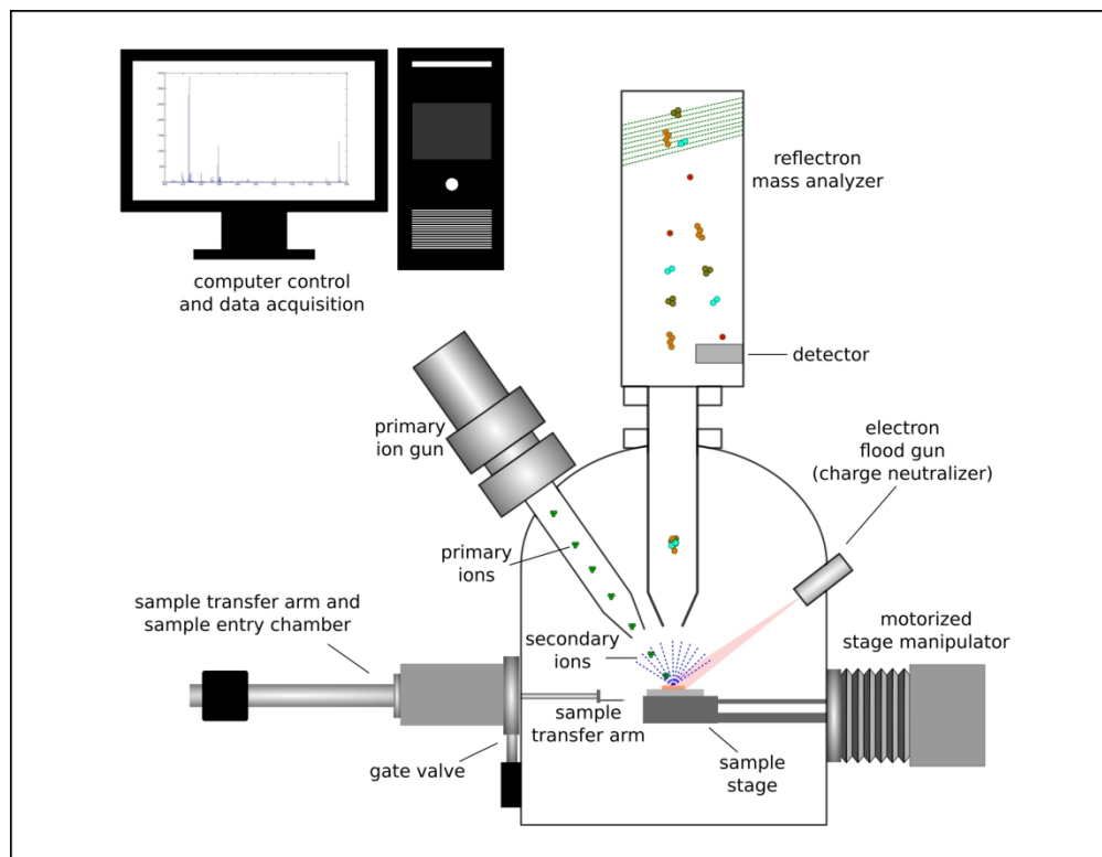
Schematic drawing of a ToF-SIMS instrument.
