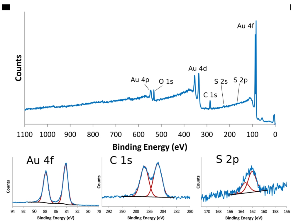
XPS survey scan (top panel) and XPS high resolution peaks for Au4f (bottom left panel), C1s (bottom middle panel) and S2p (bottom right panel). Red lines show the individual peaks for each peak fit.
