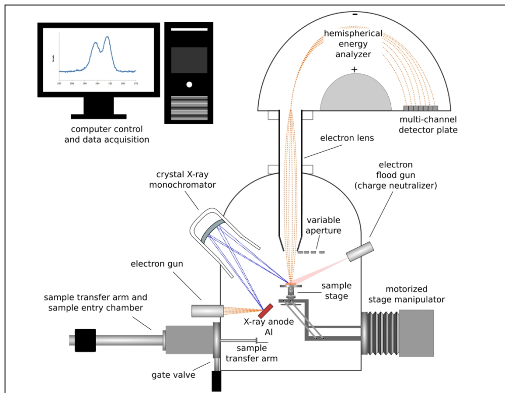
Schematic drawing of a monochromatized XPS instrument with a hemispherical analyzer and multi-channel detector.
