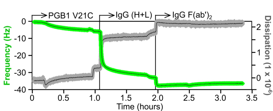
QCM-D sensorgram showing sequential immobilization of Protein G B1 cysteine mutant (V21C), whole IgG and IgG F(ab') 2 fragment onto a maleimide terminated OEG SAM. The green trace represents the frequency change and the gray trace represents the dissipation change.
