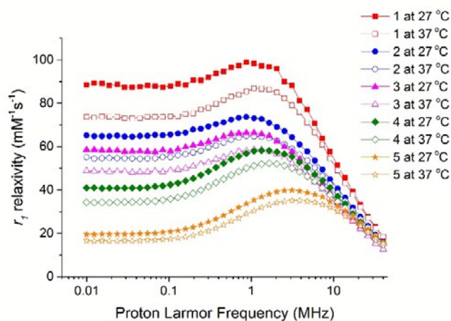
Figure 7. ^1\text{H} NMRD profiles for heparin-stabilised \text{Fe}_3\text{O}_4 nanoparticles, prepared according to Table 1. The r_1 values have been calculated in terms of [\text{Fe}] content of the samples. Profiles have been measured at two different temperatures, representative of room temperature (27 °C) and body temperature (37 °C).
