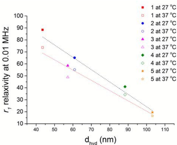
Figure 8. Low frequency relaxivity ( r_1 at 0.01 MHz at 27 °C (filled symbols) and 37 °C (open symbols)) of heparin-stabilised Fe 3 O 4 nanoparticles plotted as a function of hydrodynamic diameter ( d_{\text{hyd}} ). Dotted lines represent a linear fit of data collected at 27 °C (black) and 37 °C (red).
