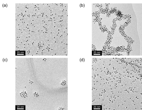
Fig. 5 Assembly and disassembly of covalently linked NP aggregates. TEM images of: (a) AuNP- 1 ; (b) assembly formed on treating AuNP- 1 with bifunctional linker 6 ; (c) colloidal stable discrete assemblies observed after treating the fully precipitated aggregate in (b) with 1,2-dihydroxybenzene for 35 days; (d) fully disaggregated AuNPs formed from (b) after a total of 42 days in the presence of 1,2-dihydroxybenzene. For several more images of each stage, see ESI † .
