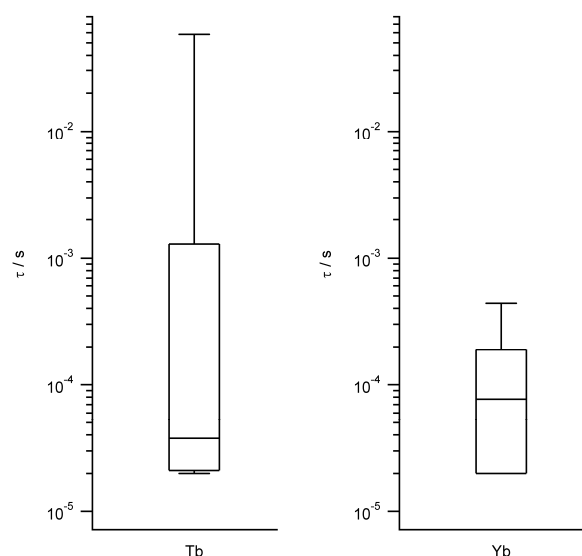
Figure 4: Box plots with the full distribution of estimates decoherence times \tau for diverse LBT structures substituted by Tb (left) and Yb (right).
