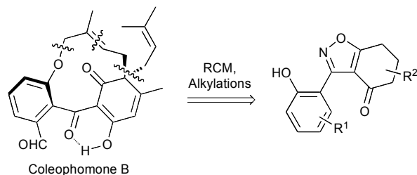
Scheme 1. Strategic disconnection of coleophomones
