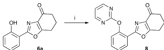
Scheme 4. Reagents: i, 2-chloropyrimidine, Cs 2 CO 3 , Cu, dry DMF, 1 day
