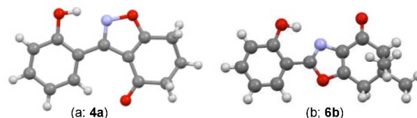
Fig. 1a and 1b. X-Ray crystal structures of isoxazole 4a and oxazole 6b (O = red, N = blue, C = grey, H = light grey).
