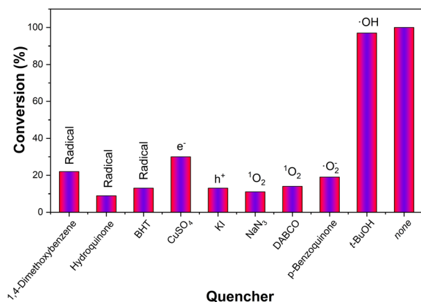
Fig. 2 The effect of quenchers on the photooxidation of thioanisole (1a) to sulfoxide 2a, using FG as a photochemical promoter. The reaction was performed with thioanisole (1a) (25 mg, 0.20 mmol), FG (1 mg) in MeOH (0.5 mL), under Blue LED irradiation (Kessil PR160L, 456 nm). FG was obtained after 30 minutes of sonication of GrF (1 mg) in the reaction's solvent, before the addition of 1a and quencher. Conversion was determined by 1 H-NMR.
