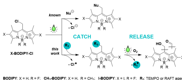
Scheme 1 Catch-and-release photoreactivity of BODIPY–Cl.
