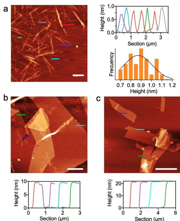
Fig. 4 Atomic force microscopy images. a) ^6\text{CP} nanotubes isolated by sonication with height profiles and size distribution ( n=30 ) on the right; scale bar = 2 \mu\text{m} . b-c) ^6\text{CP} nanosheets with height profiles shown below each image; scale bars = 3 \mu\text{m} (b) 10 \mu\text{m} (c). All samples were prepared at pH 6.5.
