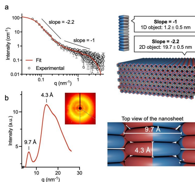
Fig. 5 X-ray scattering analyses of ^6\text{CP} samples. a) SAXS profile fitted to a combination of a cylindrical and a lamellar model, 64 consistent with coexisting 1D nanotubes and 2D nanosheets. b) WAXS profile, showing spacings at 9.7 and 4.3 Å, in agreement with the expected packing of cyclic peptide monomers as laterally-interfacing nanotubes. All samples were prepared at pH 6.5.
