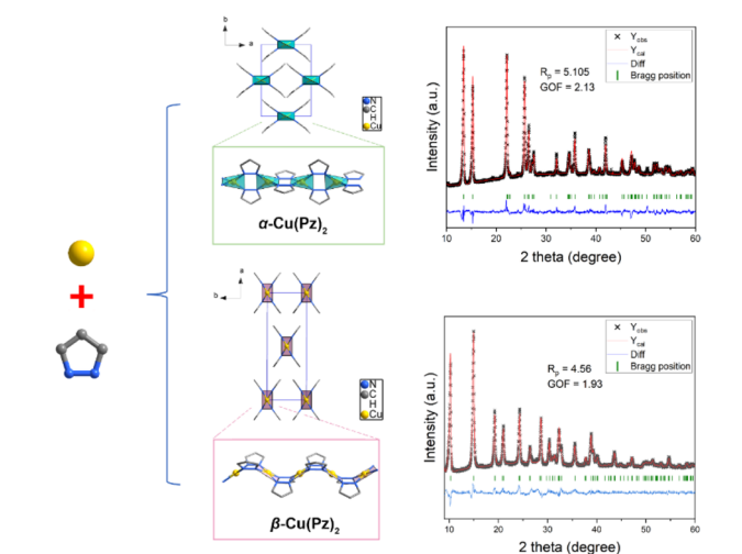
Fig. 1 Illustration of crystal structures of \alpha - Cu(Pz) 2 and \beta - Cu(Pz) 2 and the corresponding Rietveld refinement patterns.
