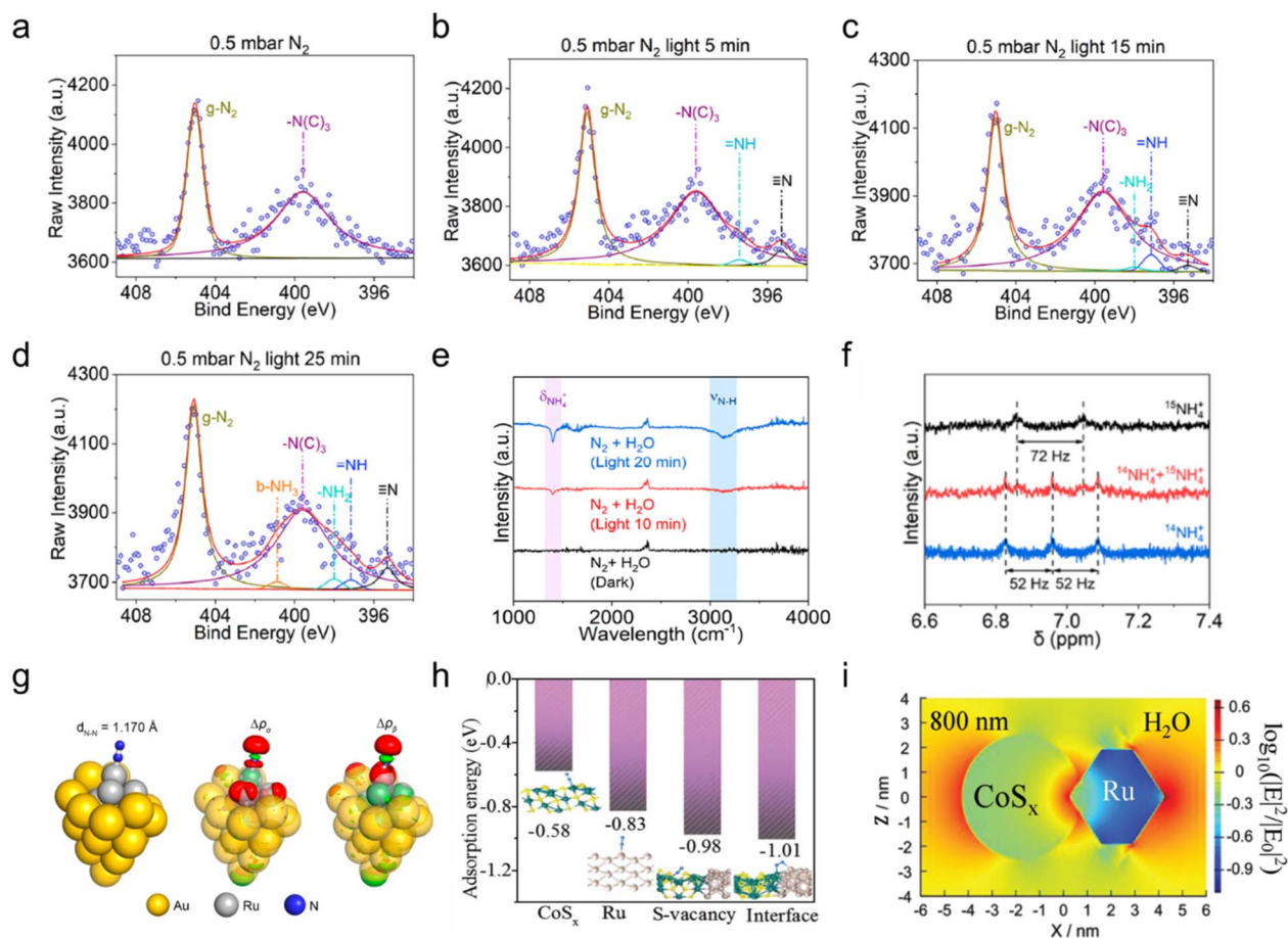
Fig. 12 (a)–(d) N 1s XPS spectra of AuRu 0.31 . (e) In situ DRIFTS spectra recorded for N 2 + H 2 O over AuRu 0.31 under irradiation conditions. (f) 1 H NMR spectra of solution after the N 2 fixation reaction in the 15 N 2 , 15 N 2 + 14 N 2 , or 14 N 2 atmosphere. (g) Optimized structures of N 2 adsorbed on the AuRu cluster. Reproduced with permission. 82 Copyright 2019, American Chemical Society. (h) Adsorption energies of N 2 on different sites. FDTD electric field distribution. (i) FDTD electric field distribution at Ru/CoS x nanoparticle (800 nm irradiation) observed from γ-axis (vertical to incident light). Reproduced with permission. 83 Copyright 2019, Wiley-VCH.
