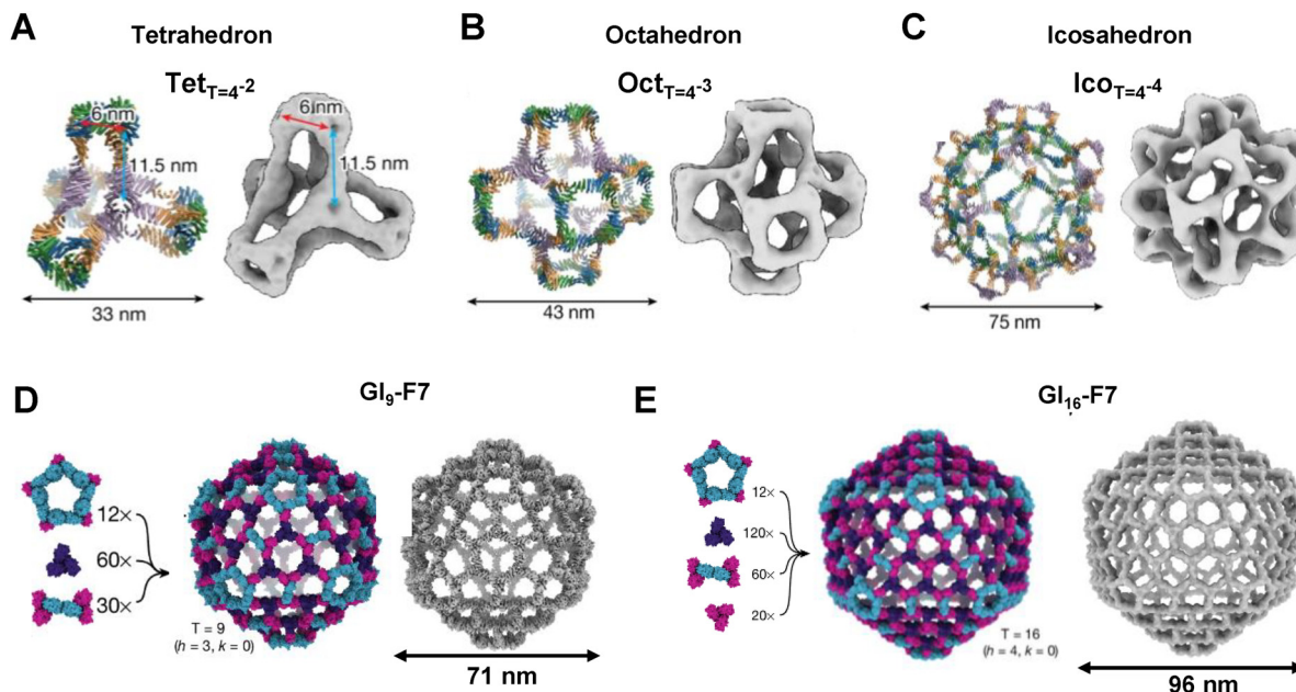
Fig. 4 Protein nanocages designed by programmed symmetry breaking: (A) a tetrahedral nanocage ( Tet_{T=4} ) composed of 48 subunits, (B) an octahedral nanocage ( Oct_{T=4} ) with 96 subunits, and (C) an icosahedral nanocage ( Ico_{T=4} ) containing 240 subunits. (D) A 540-subunit nanocage ( GI_9 -F7) assembled from 12 pentasymmetrons, 60 cyclic C3 (CCC) homotrimers, and 30 dissymmetrons. (E) A 960-subunit nanocage ( GI_{16} -F7), constructed from the same modular components, was visualized by low-resolution cryo-EM. Note: GI_T -X, where G stands for Goldberg, I for icosahedral symmetry, T is used to denote the triangulation number of a particular architecture, and X is a unique identifier for each design.
