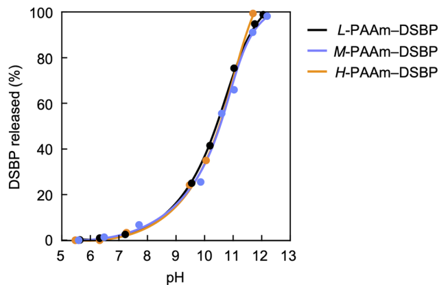
Fig. 11 Release efficiency of DSBP as a function of pH, determined from UV absorbance at \lambda = 348 nm.
