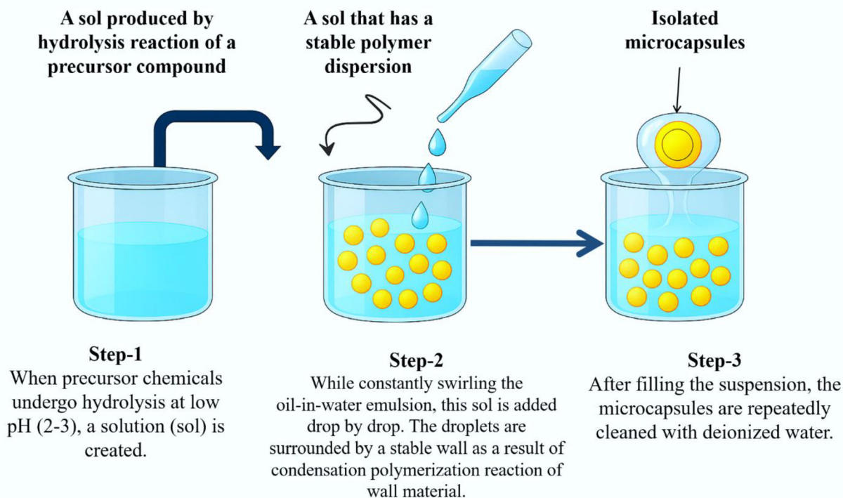
Fig. 7 Sol-gel technique for microcapsule production showing transformation from colloidal sol to solid gel encapsulating healing agent, producing capsules of 100–500 \mu\text{m} .
