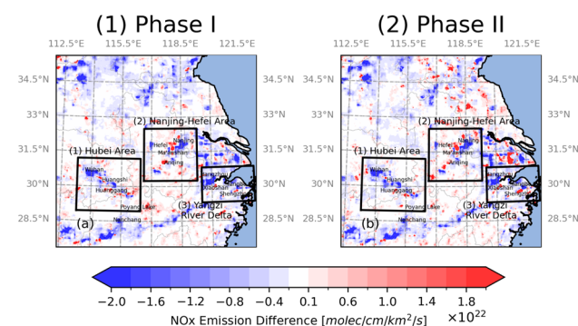
Fig. 2 Spatial distribution of NO x emission differences between lockdown phases and pre-lockdown baseline over eastern China. (a) Phase I (strict lockdown) and (b) Phase II (early recovery) emission changes. Black boxes denote three study regions: (1) Region I: Hubei Area, (2) Region II: Nanjing–Hefei Area, and (3) Region III: Yangtze River Delta. Negative values (blue) indicate emission reductions; positive values (red) indicate increases.
