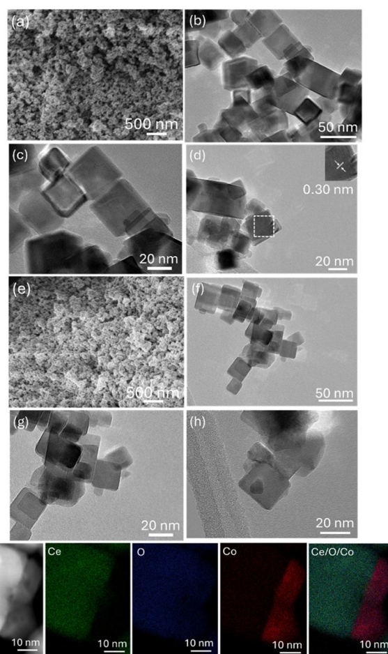
Fig. 5 SEM and HRTEM images of CeO 2 -NC (a–d) and Co/CeO 2 -NC (e–h), (i) HAADF-STEM spectra and corresponding EDS elemental mapping of Co/CeO 2 -NC. The inset in Fig. 5d shows a magnification of the lattice fringes.
