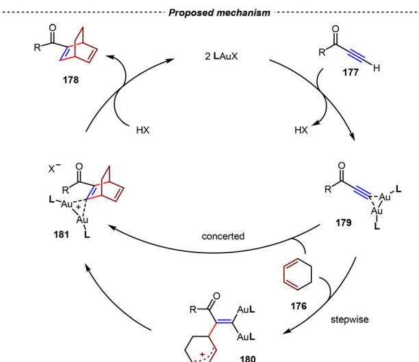
Scheme 39 Au(I)/phosphoramidite-catalyzed asymmetric intermolecular [4+2] cycloadditions of ynones and cyclohexa-1,3-dienes.
