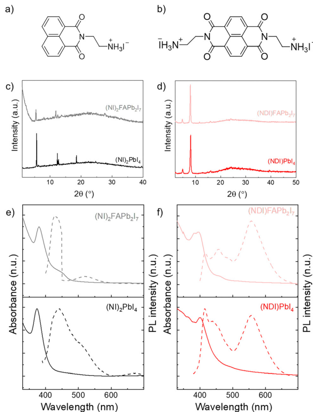
Fig. 1 Structural and optoelectronic properties of naphthal(enedi)imide LD perovskites. (a) and (b) Structural representations of NI and NDI. (c) and (d) XRD patterns of films of (c) (NI)_2PbI_4 , (NI)_2FAPb_2I_7 , (d) (NDI)PbI_4 , and (NDI)FAPb_2I_7 nominal compositions. (e) and (f) UV-Vis (full line) and PL (dashed line) spectra of films based on (e) (NI)_2PbI_4 , (NI)_2FAPb_2I_7 , (f) (NDI)PbI_4 , and (NDI)FAPb_2I_7 nominal compositions on glass.
