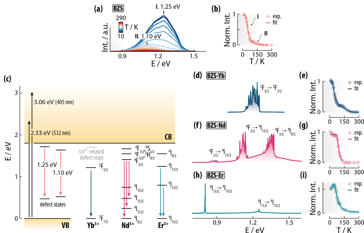
Fig. 4 (a) Photoluminescence of BZS (undoped \text{BaZrS}_3 ) as a function of temperature and (b) intensity vs. temperature plot obtained integrating over the whole range shown in (a). (c) Proposed energy level scheme for the doped and undoped samples. For \text{Ln}^{3+} ions, only the energy levels that are in the range <1.8 eV are shown. The emission spectra recorded at 10 K for BZS-Yb, BZS-Nd, and BZS-Er are shown in (d), (f), and (h), alongside the intensity vs. temperature plots obtained for each sample – shown respectively in (e), (g), and (i). Details about the data treatment for obtaining the integrated intensity for (e), (g), and (i) can be found in the ESI†. All the fittings were carried out using eqn (1). All spectra were collected under 405-nm excitation, save for the BZS-Yb sample, which was excited at 532 nm.
