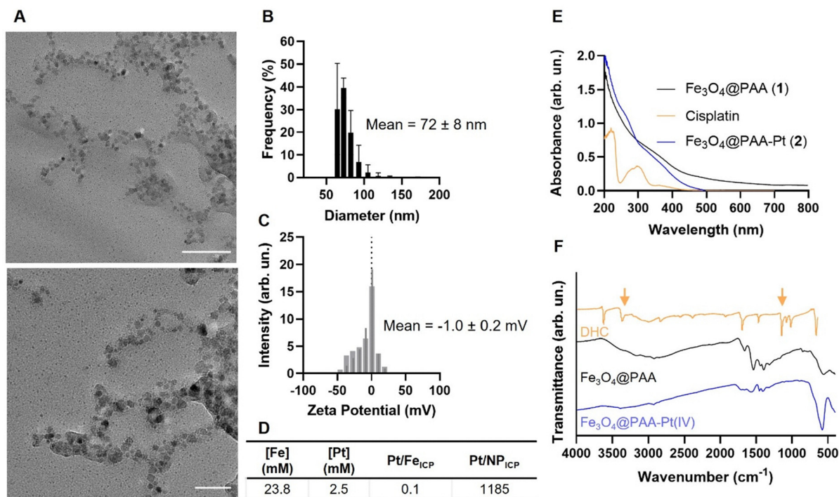
Fig. 3 (A) Representative bright-field TEM images of \text{Fe}_3\text{O}_4@PAA-Pt(IV) NPs, with scale bar representing 100 nm (above) and 50 nm (below). (B) Size distribution of nanoparticles' hydrodynamic size, as measured by DLS, in \text{H}_2\text{O} (pH = 7.4) and (C) zeta potential measurements. (D) Table summarising ICP results. (E) UV-Vis spectra of NPs 1 , 2 and cisplatin, in \text{H}_2\text{O} (pH = 7.4). (F) FTIR spectra of NPs 1 , 2 and Pt(IV) complex (DHC).
