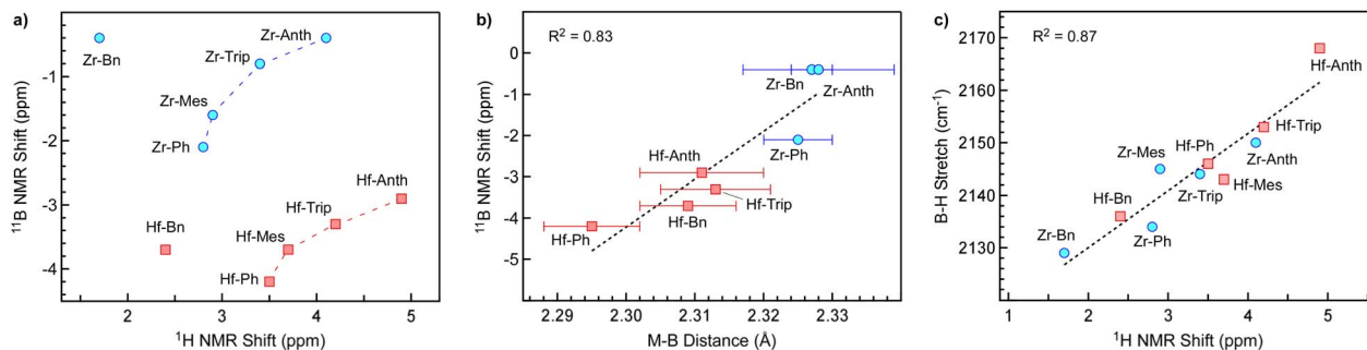
Fig. 4 Spectroscopic comparisons for [M(RBH_3)_4] complexes with M = Zr (blue circles) or Hf (red squares). (a) Comparison of ^1H and ^{11}B NMR shifts assigned to BH_3 resonances in C_6D_6 at RT. The dashed lines are shown to emphasize the trends between the data points for complexes with different aryl substituents. (b) Comparison of ^{11}B NMR shifts to M-B distances from single-crystal XRD studies. Error bars denote the standard deviation of the average M-B distances. (c) Comparison of the higher energy B-H stretches obtained from the IR spectra to ^1H NMR shifts for the BH_3 resonances. The black dashed line in panels (b) and (c) is the linear fit to all data points shown.
