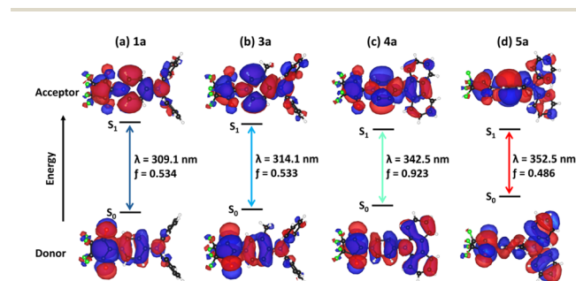
Fig. 7 Natural transition orbitals, vertical transition energies ( \lambda ), and oscillator strengths ( f ) calculated in the gas phase for the S_0 \rightarrow S_1 transition in (a) 1a ; (b) 3a ; (c) 4a ; and (d) 5a . Calculations were performed at the \omega\text{B97xD3} def2-TZVP level, on crystal coordinates. Iso-surface values are 0.01.
