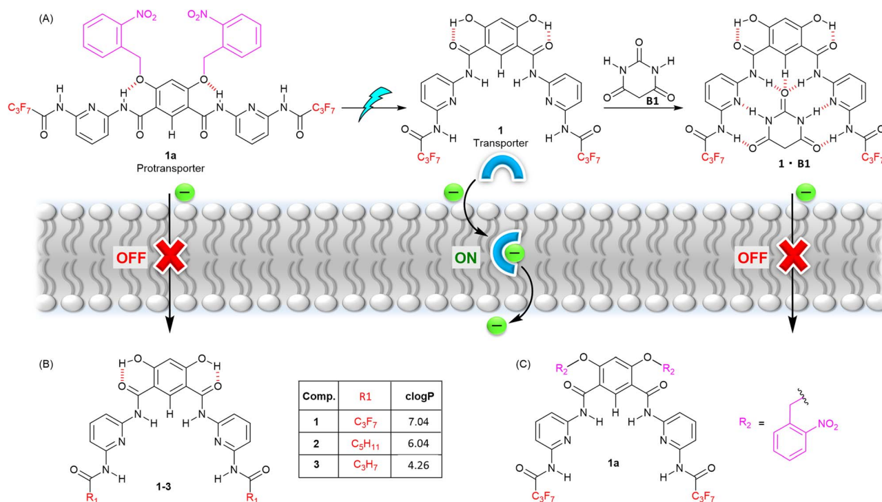
Fig. 1 (A) Schematic representation of stimuli-responsive anion transport. (B) Chemical structure of transporters 1–3 , with \text{clogP} values calculated using MarvinSketch. (C) Caged pro-transporter 1a .
