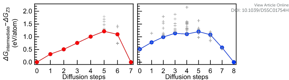
Fig. 7 Formation energies, or Gibbs free energies at 0 K, of intermediate structures ( \Delta G_{\text{intermediate}} ) compared with Z3- \text{Fe}_8\text{Pd}_{20}\text{In}_4 ( \Delta G_{\text{Z3}} ), where the red and blue curves are the diffusion paths with the minimum formation energies formed from \text{L}_{12}\text{-Fe}_4\text{Pd}_{24}\text{In}_4 and \text{L}_{10}\text{-Fe}_{16}\text{Pd}_{16}/\text{bct-Pd}_{24}\text{In}_8 , respectively, and the + mark represents other paths.
