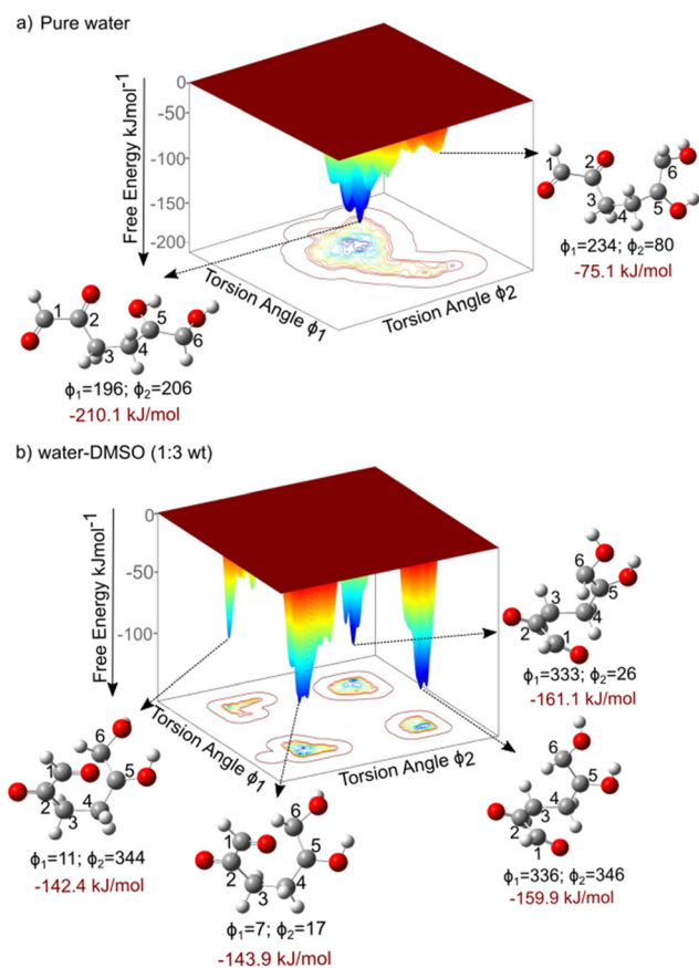
Fig. 3 Free energy landscape of the conformational analysis of 5,6-enol, computed using CPMD–metadynamics simulations. The free energy is computed as a function of dihedral angles in degrees, with explicit solvent molecules treated quantum mechanically. a) Pure water and b) water–DMSO mixture (1,3 mass ratio). Refer to Fig. 1 for the definitions of the collective variables CV_1 and CV_2 . Free energies ( \Delta G_R ) are reported in \text{kJ mol}^{-1} .
