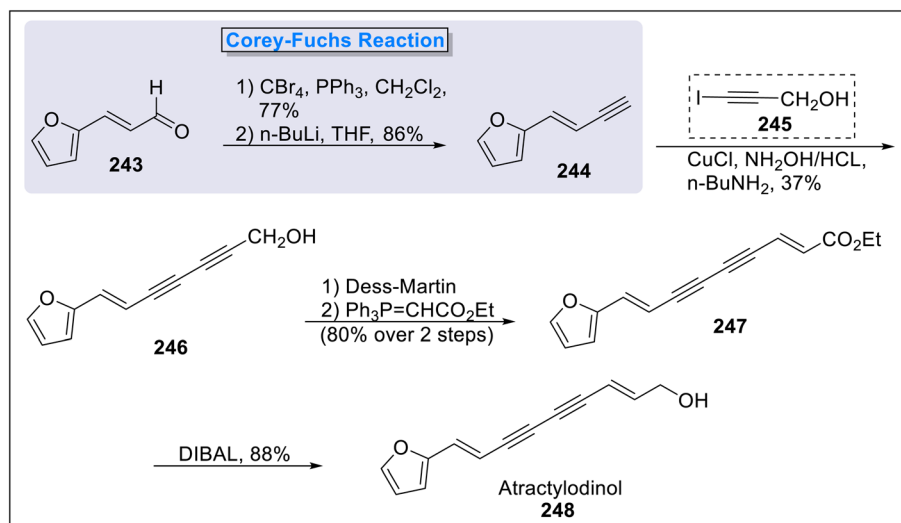
Scheme 24 Total synthesis of atractylodinol 248 by Kraus and coworkers.
