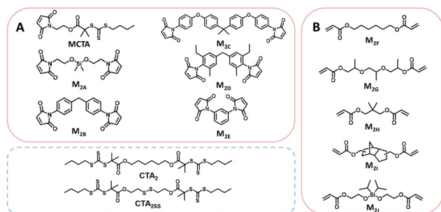
Scheme 2 Monomers discussed in this work: (A) maleimides and (B) acrylates.
