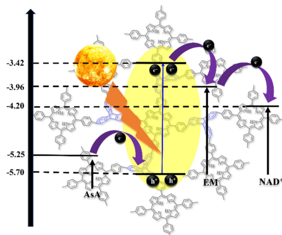
Scheme 2 Potential energy diagram of the photocatalytic pathway.
