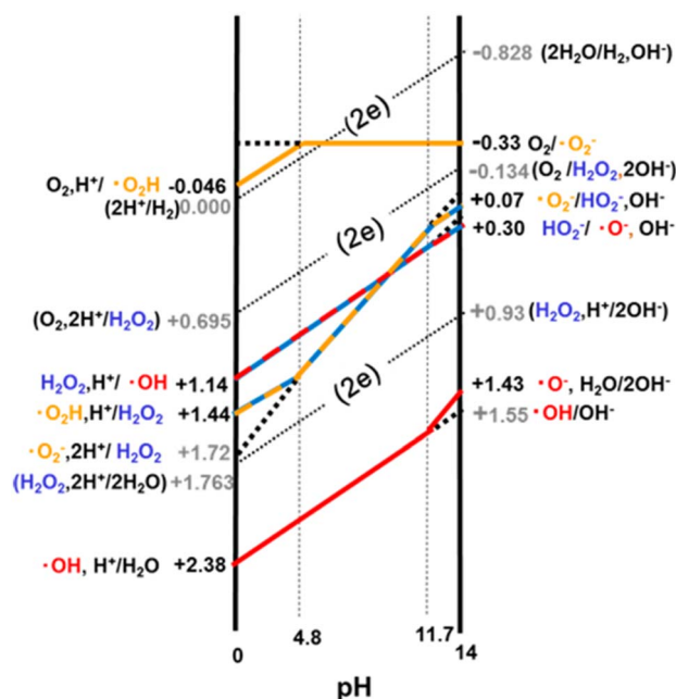
Fig. 2 The pH dependence of one-electron redox reactions involving H 2 O (water), H 2 O 2 (hydrogen peroxide), and O 2 (oxygen). The dotted line in the graph indicates a two-electron (2e) process. 54
