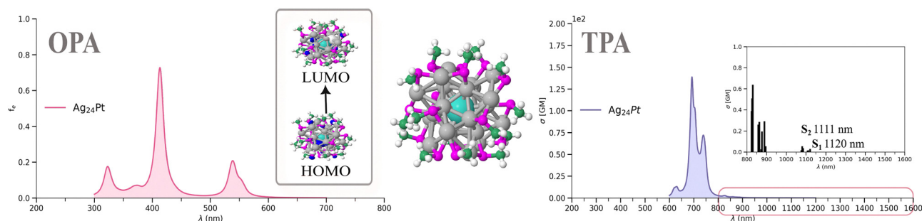
Fig. 3 TDDFT OPA (left) and TPA 71–73 (right) spectra calculated at the CAM-B3LYP 74 /def2-SVP 75 level of theory for PtAg 24 (SCH 3 ) 18 . For the Pt and Ag atoms the 19-electron relativistic effective core potential (19-e RECP) developed by the Stuttgart group 76 was implemented. DFT optimized structure with centrally doped single Pt atom is shown at the center, as well as HOMO–LUMO analysis. Atoms are colored by element: Ag in grey, Pt in turquoise, S in magenta, C in green, and H in white.
