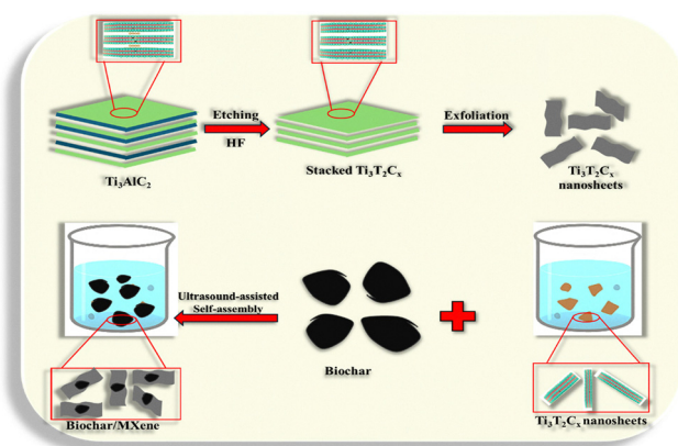
Fig. 8 Biochar/MXene fabrication strategy.
