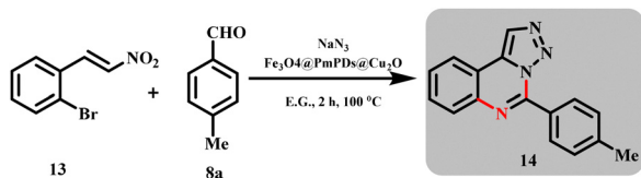
Scheme 6 \text{Fe}_3\text{O}_4 @poly( m -phenylenediamines)@ \text{Cu}_2\text{O} catalysed synthesis of quinazolinones (Rawat et al. ).
