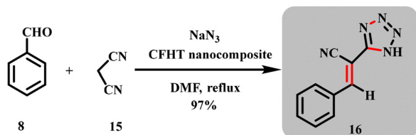
Scheme 7 Catalytic synthesis of 5-substituted 1 H -tetrazole derivatives (Hajjizadeh et al. ).
