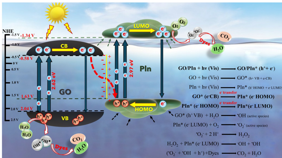
Fig. 13 Plausible photocatalytic mechanism of dye degradation by the GO/PIIn composite: diagrammatic representation and proposed pathway scheme.
