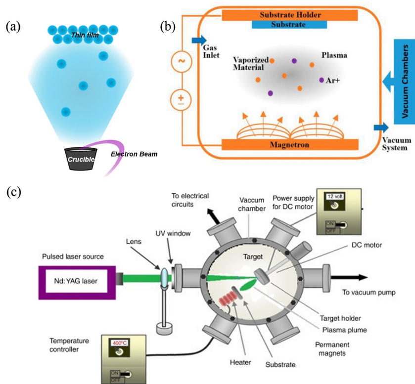
Fig. 15 Schematic illustration of the (a) EB-PVD, (b) sputtering, (c) PLD. 244,268,309 Reproduced from ref. 244 with permission from [Springer], copyright [2020]. Reproduced from ref. 309 with permission from [MDPI], copyright [2023].
