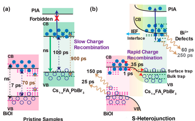
Fig. 6 (a) Depiction of kinetic models for (a) pristine BiOI and \text{Cs}_{1-x}\text{FA}_x\text{PbBr}_3 (CF) and (b) hybrid \text{Cs}_{1-x}\text{FA}_x\text{PbBr}_3:\text{BiOI} (CF:BiOI) heterojunction samples. IEF represents the internal electric field generated in the heterojunction. Reprinted with permission from ref. 106. Copyright 2022, American Chemical Society.
