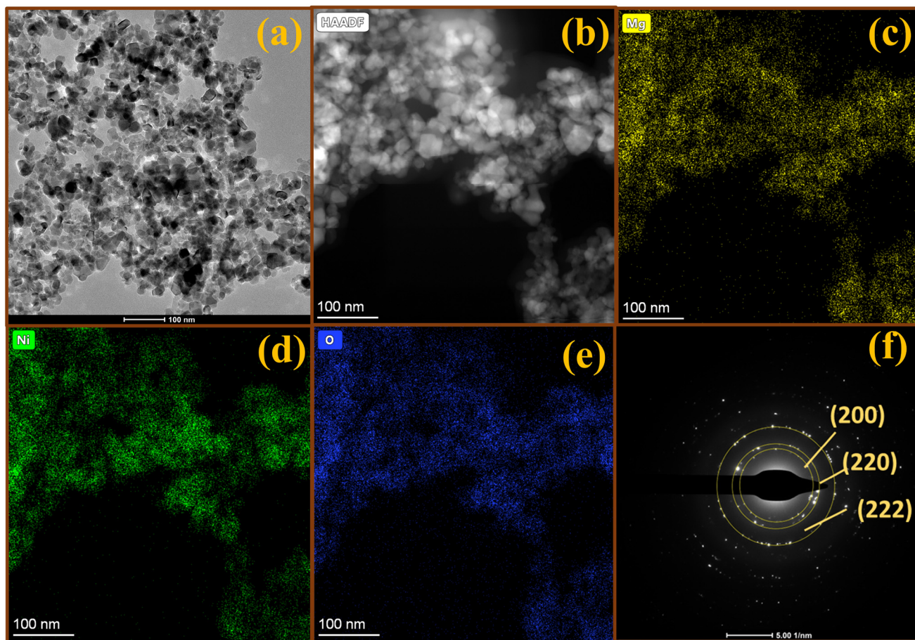
Fig. 1 (a) TEM micrographs of the MgNiO _2 particles representing the well-ordered crystalline structure. (b) HAADF image of the MgNiO _2 . (c–e) Atomic mapping of Mg, Ni and O. (f) SAED patterns of the MgNiO _2 nanoparticles.
