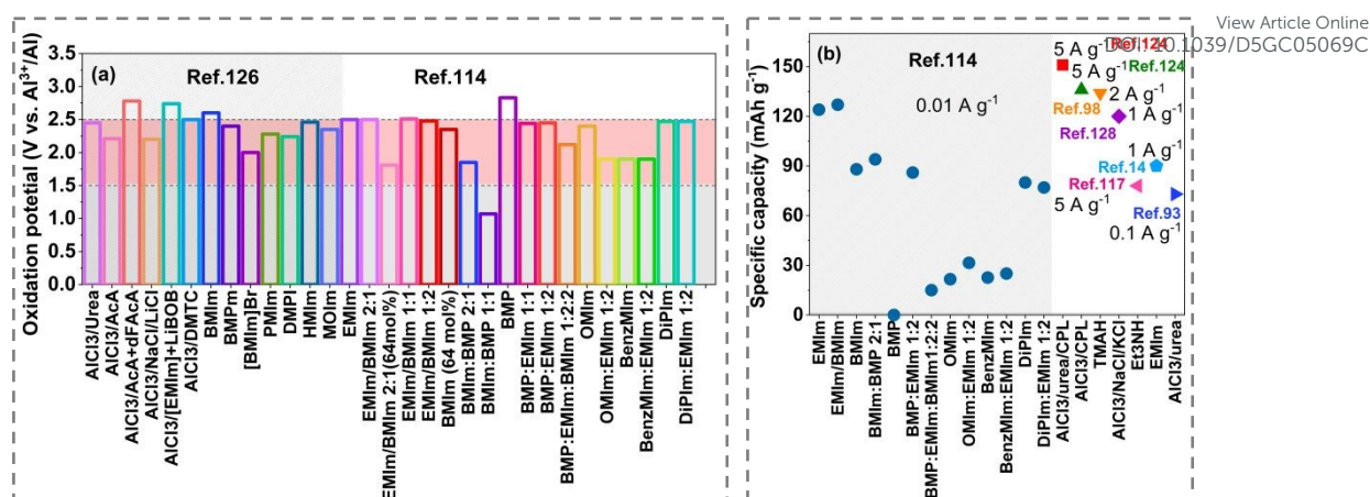
Figure 14. a) The oxidation onset potentials of various \text{AlCl}_3/[\text{X}]\text{Cl} and other alternative electrolytes. 114,126 b) Specific capacities of \text{Al}/\text{graphite} cells with various \text{AlCl}_3/[\text{X}]\text{Cl} and other alternative electrolytes. \text{AlCl}_3/[\text{X}]\text{Cl} ( \text{X} = \text{EMIm} to \text{DiPIm} : \text{EMIm} 1:2) at 0.01 \text{A/g}^{114} , \text{AlCl}_3/\text{urea}/\text{CPL} and \text{AlCl}_3/\text{CPL} at 5 \text{A/g}^{124} , \text{AlCl}_3/\text{TMAHCl} at 2 \text{A/g}^{98} , \text{AlCl}_3/\text{NaCl}/\text{KCl} at 1 \text{A/g}^{128} , \text{AlCl}_3/\text{Et}_3\text{NHCl} at 5 \text{A/g}^{117} , \text{AlCl}_3/[\text{EMIm}]\text{Cl} at 1 \text{A/g}^{14} , and \text{AlCl}_3/\text{urea} at 0.1 \text{A/g}^{93} . Adapted with permission from American Chemical Society 114 . Copyright 2023. Adapted with permission from John Wiley and Sons 126 . Copyright 2023.
