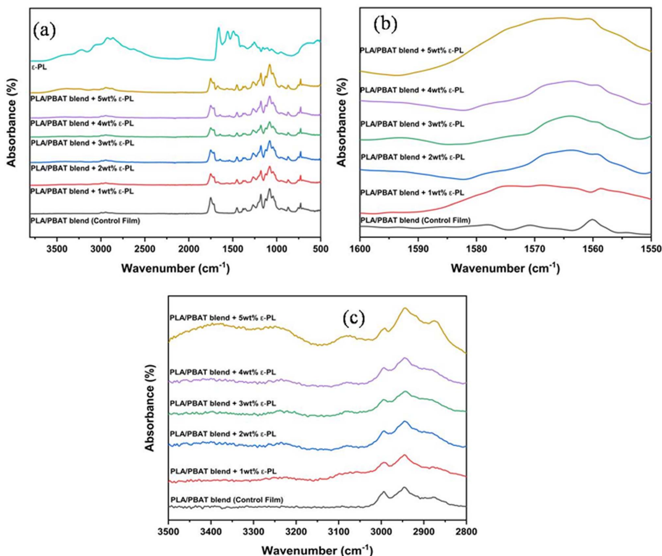
Fig. 1 (a) FTIR spectra of \epsilon -PL, PLA/PBAT blend control film and PLA/PBAT blend films loaded with different weight percentages of \epsilon -PL (1–5 wt%). (b) Enlarged view of the FTIR spectra in the 1550\text{--}1600 \text{ cm}^{-1} regions. (c) Enlarged view of the FTIR spectra in the 2800\text{--}3500 \text{ cm}^{-1} regions.
