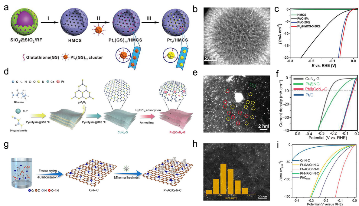
Fig. 5 (a) Schematic illustration of the synthetic procedure of Pt 5 /HMCS. Step I: carbonization and etching of SiO 2 to form HMCS. Step II: load the Pt 5 (GS) 10 clusters into HMCS to form Pt 5 (GS) 10 /HMCS. Step III: conversion of Pt 5 (GS) 10 /HMCS to Pt 5 /HMCS electrocatalyst through thermal treatment. (b) HAADF-STEM image. (c) LSV curves of Pt 5 /HMCS-5.08% and commercial Pt/C (5 and 20 wt%) catalysts based on the geometric area of the working electrode in 1.0 M KOH. Reproduced with permission. 112 Copyright 2019, Wiley-VCH GmbH. (d) Synthetic illustration of the synthetic process for Pt@CoN 4 -G. (e) Aberration-corrected HAADF-STEM image. Single Co atoms are marked by yellow circles, and single Pt atoms are marked by red circles. (f) LSV curves of different electrocatalysts in 1.0 M KOH. Reproduced with permission. 113 Copyright 2023, Wiley-VCH GmbH. (g) Schematic illustration of the preparation of Pt-AC/Cr-N-C. (h) HAADF-STEM image. Inset, the size distribution of Pt ACs. (i) LSV curves tested in 1 M KOH solution. Reproduced with permission. 114 Copyright 2023, American Chemical Society.
