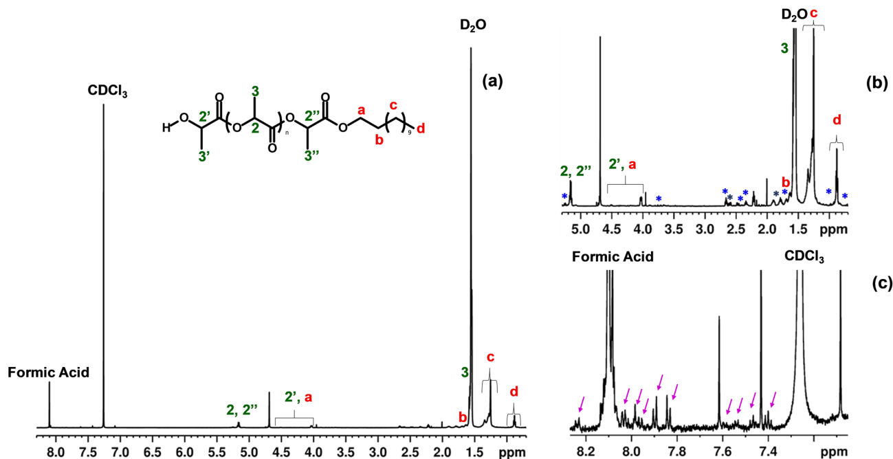
Fig. 6 (a) The ^1\text{H} NMR spectra of the PLA NPs in \text{CDCl}_3 . Inset: the molecular structure of PLA. The numbers indicate the methyl ( -\text{CH}_3 ) and methenyl ( =\text{CH}- ) protons backbone, and the letters correspond to the protons of the lactic acid unit bearing the hydroxyl end group. (b) Zoom-in of the aliphatic region; blue (*) indicates possible signals of PLA of different chain lengths. (c) Zoom-in of the aromatic region; purple arrows indicate some signals of aromatic compounds.
