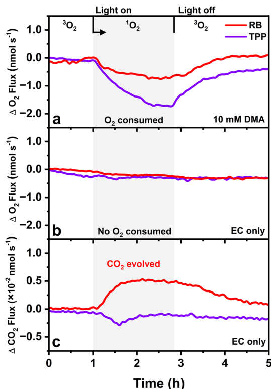
Fig. 4 OMS analysis demonstrating that ethylene carbonate itself is stable to ^1\text{O}_2 and that CO 2 release is coupled to the photocatalyst instability. (a) Change in O 2 (32 m/z ) flux for solutions of 10 mM DMA in EC showing ^1\text{O}_2 is generated and reacting with DMA when illuminated; (b) change in O 2 (32 m/z ) flux for EC solutions showing no notable reactivity of ^1\text{O}_2 ; (c) change in CO 2 (44 m/z ) flux for EC solutions indicating CO 2 release for reactions containing RB but not TPP. All EC solutions contained 10 \mu\text{M} of photocatalyst (RB: red line; TPP: purple line) and a constant flow of 20% O 2 in Ar gas was used during OMS measurements.
