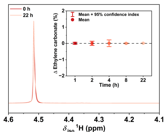
Fig. 5 ^1\text{H} NMR spectra of ethylene carbonate after long-term exposure to ^1\text{O}_2 showing no detectable reaction between EC and ^1\text{O}_2 . 0.1 M EC with 100 \mu\text{M} TPP in CDCl 3 under an atmosphere of O 2 was illuminated by a red LED lamp (40 W) for 22 hours. Intensities corrected to the internal standard (dimethyl sulfone). (inset) A plot showing no relevant percentage change in moles of EC over the course of this reaction. Aliquots were taken for analysis by quantitative ^1\text{H} NMR spectroscopy. This reaction was conducted in duplicate and results from the two reactions averaged.
