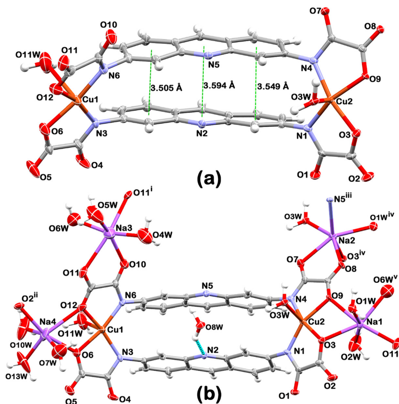
Fig. 1 (a) A perspective view of the [3,3] metallacyclophane-type dicopper(II) fragment in 1. Here and in the next picture, green dashed lines denote the \pi\cdots\pi interactions (the displayed distances were measured between the centroids calculated through each one of the three six-ring atoms of the acridine moiety). (b) A view of the dicopper(II) metallacyclophane's assembling role towards the sodium ions shows the coordination environment of the four crystallographically independent alkaline cations. Cyan dashed line outlines the hydrogen bond between one water molecule of crystallization and the acridine-nitrogen atom here and in the next picture. O13W and O14W belong to the same disordered water molecule and are in 60 and 40% occupancy sites, respectively, but O14 and its hydrogen atoms were omitted for clarity in this panel. In both panels and in panel (a) of the next picture, all non-hydrogen atoms were drawn at the 30% probability level, whereas the hydrogen atoms are represented with spheres of arbitrary radius. Carbon and hydrogen atoms were not labelled [Symmetry code: (i) = -x, \frac{1}{2} + y, 1 - z ; (ii) = x, y, -1 + z ; (iii) = -x, \frac{1}{2} + y, 2 - z ; (iv) = x, 1 + y, z ; (v) = x, y, 1 + z ].
