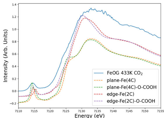
Fig. 7 Comparison between the XANES absorption spectrum of FeOG in \text{CO}_2 flow at 433 K (continuous line) and simulated XAS spectra (dashed lines) for a selection of Fe single atom centres. Spectra have been applied a vertical offset for clarity. Atoms in parenthesis specify the in-plane atoms binding Fe in the simulated structures.
