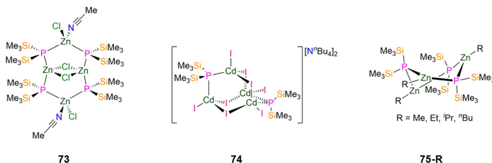
Fig. 21 Group 12 P'' cluster complexes [(Zn(Cl)(MeCN)(μ-P'')) 2 {Zn(μ-Cl)} 2 ] (73), [N''Bu 4 ] 2 [Cd 4 (I) 8 (P'') 2 ] (74), [Zn(R)(P'')] (75-R; R = Me, Et, i Pr, n Bu).
