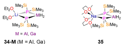
Fig. 9 Heterometallic group 13 \text{P}'' complexes [\text{M}(\text{H})_2(\mu\text{-P}''\text{Li}(\text{Et}_2\text{O})_2)]_2 ( 34-M ; M = \text{Al} , \text{Ga} ), [\text{Al}(\text{H})_2(\mu\text{-P}''\text{Na}(\text{DME})_2)]_2 ( 35 ).
