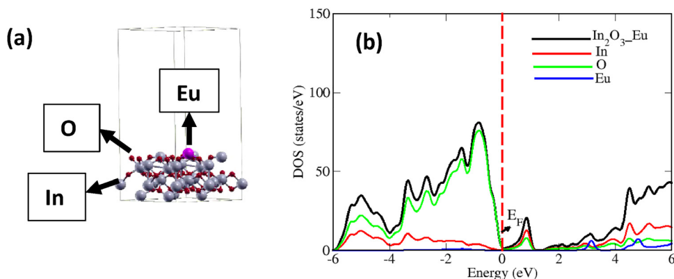
Fig. 6 (a) Optimized geometry of Eu-doped \text{In}_2\text{O}_3 obtained from DFT calculations. (b) Corresponding total and partial density of states (TDOS and PDOS) of the Eu-doped \text{In}_2\text{O}_3(001) surface.
