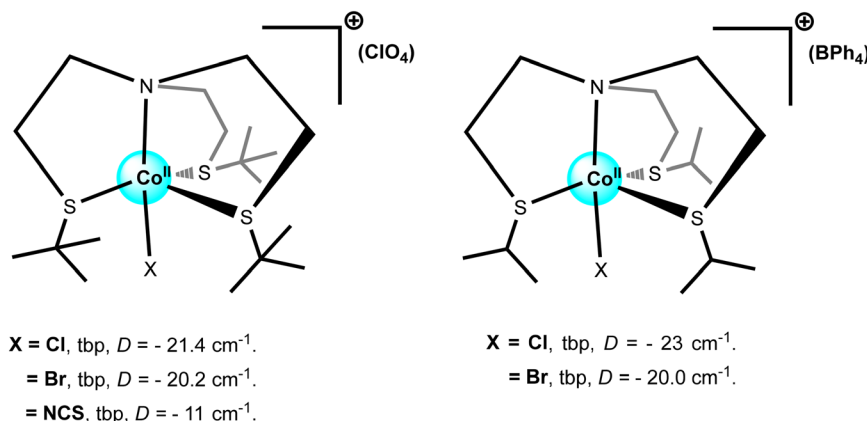
Fig. 14 Schematic representation of \text{Co}^{\text{II}} complexes 16a–16c (left) and 16d–16g (right). 88–90
