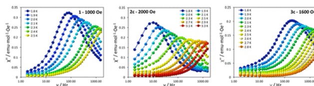
Fig. 15 Schematic representation of \text{Co}^{\text{II}} complexes 17 and 17a–17c (top) and field induced AC magnetic data for 17 , 17a and 17c at different temperatures (bottom), 91 adapted/reproduced from ref. 91 with permission from American Chemical Society, 91 copyright 2016.
