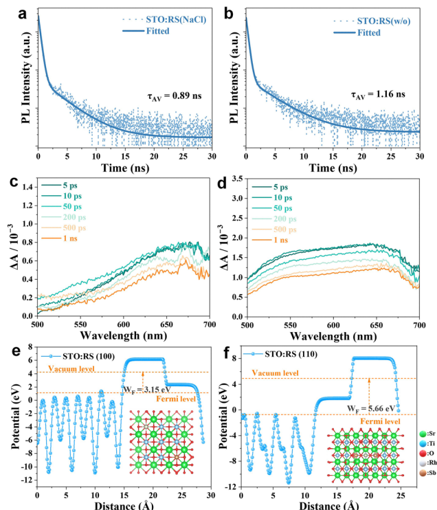
Fig. 3 TRPL decay curves of (a) STO:RS(NaCl) and (b) STO:RS(w/o) measured at 440 nm. TAS of (c) STO:RS(NaCl) and (d) STO:RS(w/o). Theoretical calculated work functions of the (e) {100} and (f) {110} facets of STO:RS(NaCl).
